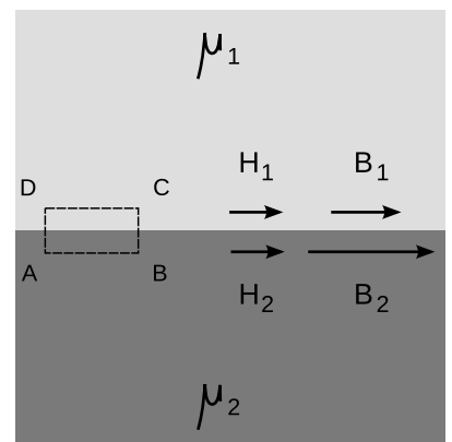
i / At a boundary between two substances with \mu_2 > \mu_1 , the \mathbf{H} field has a continuous component parallel to the surface, which implies a discontinuity in the parallel component of the magnetic field \mathbf{B} .
